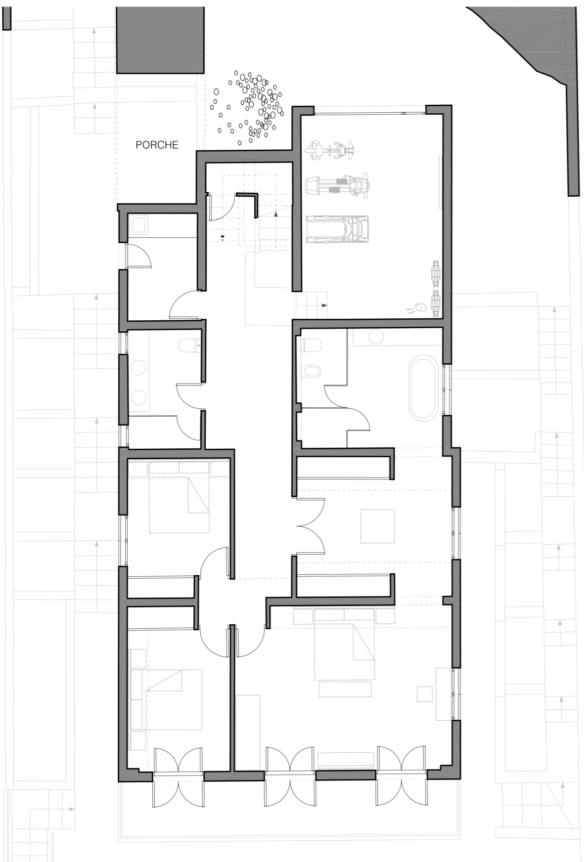
FIRST FLOOR
