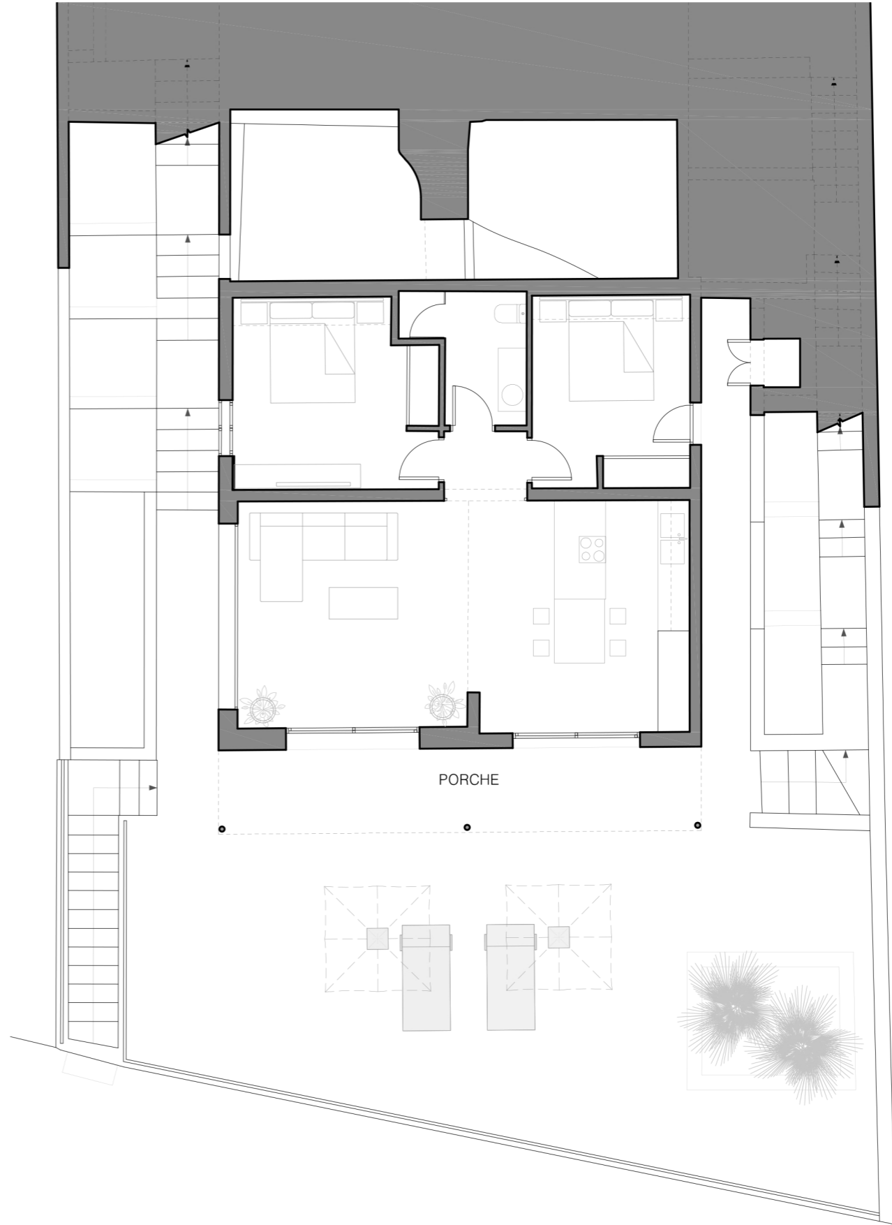
GROUND FLOOR
